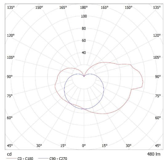
Lucis S5.L11.A350.0W ASTERION LED / LDC (Polar)
